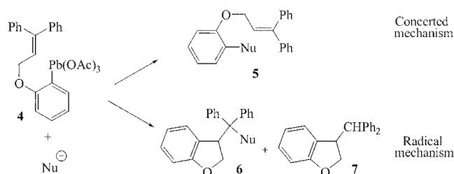
Scheme 4. Possible evolution of the reaction of organolead reagent 4 with a nucleophile
