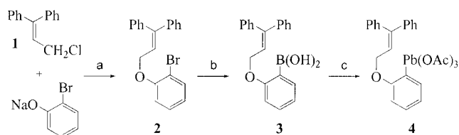
Scheme 3. Synthesis of aryllead triacetate 4 ; reagents and conditions: a) cat. NaI, THF, reflux, 6 h, 89%; b) (i) BuLi, THF, -78^\circ\text{C} , 10 min, (ii) B(OCHMe 2 ) 3 , -78^\circ\text{C} , 1.5 h, then -78^\circ\text{C} to room temp., overnight, (iii) 10% aqueous HCl, 36%; c) Pb(OAc) 4 , cat. Hg(OAc) 2 , CHCl 3 , 45^\circ\text{C} , 2 h, then room temp., 10 h, 56%.
